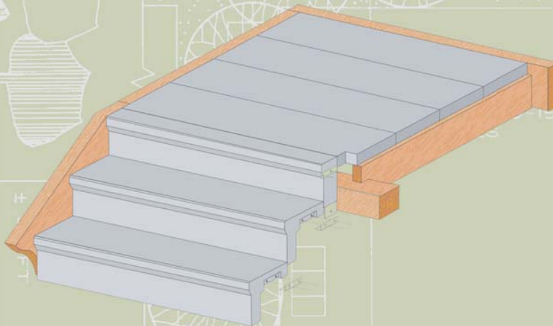
Illustration of "Bolt-on-to-Wood" framing. Attachment hardware supplied with tread order.
